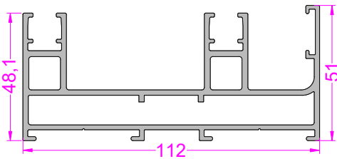
TRACK DETAILS
