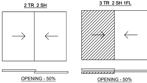
SLIDING POSSIBILITIES
