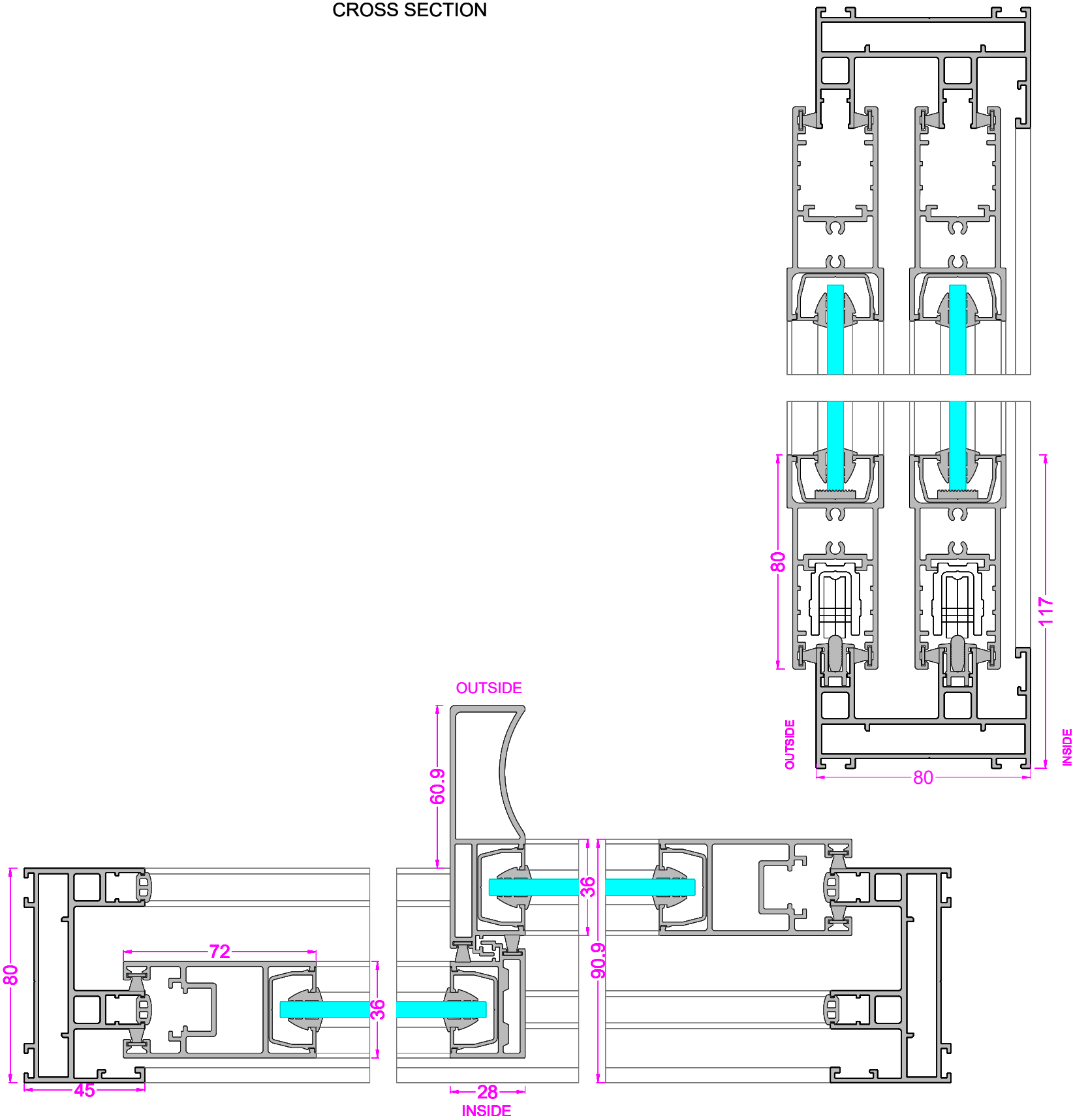
CROSS SECTION
