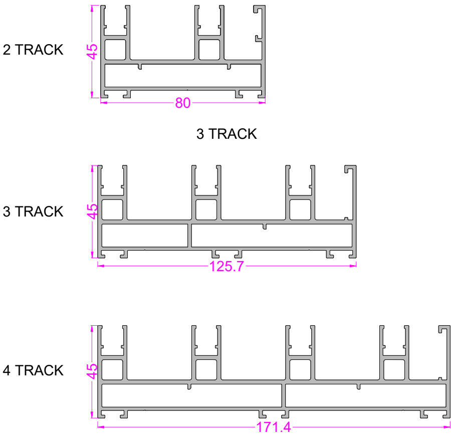
TRACK DETAILS
