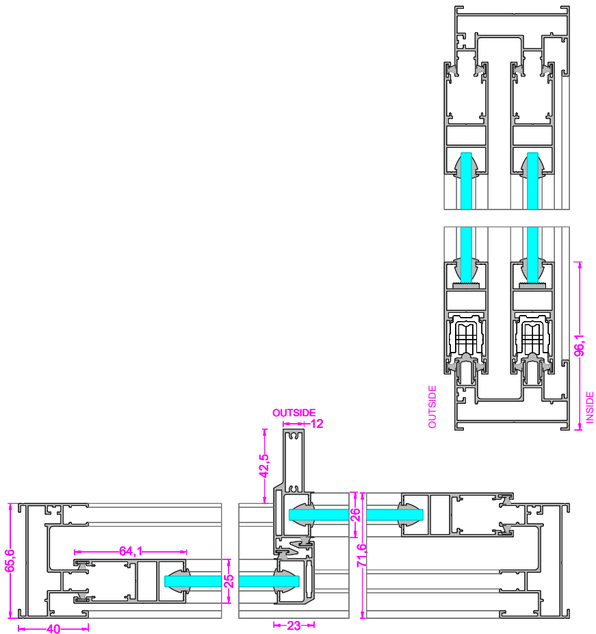
CROSS SECTION
